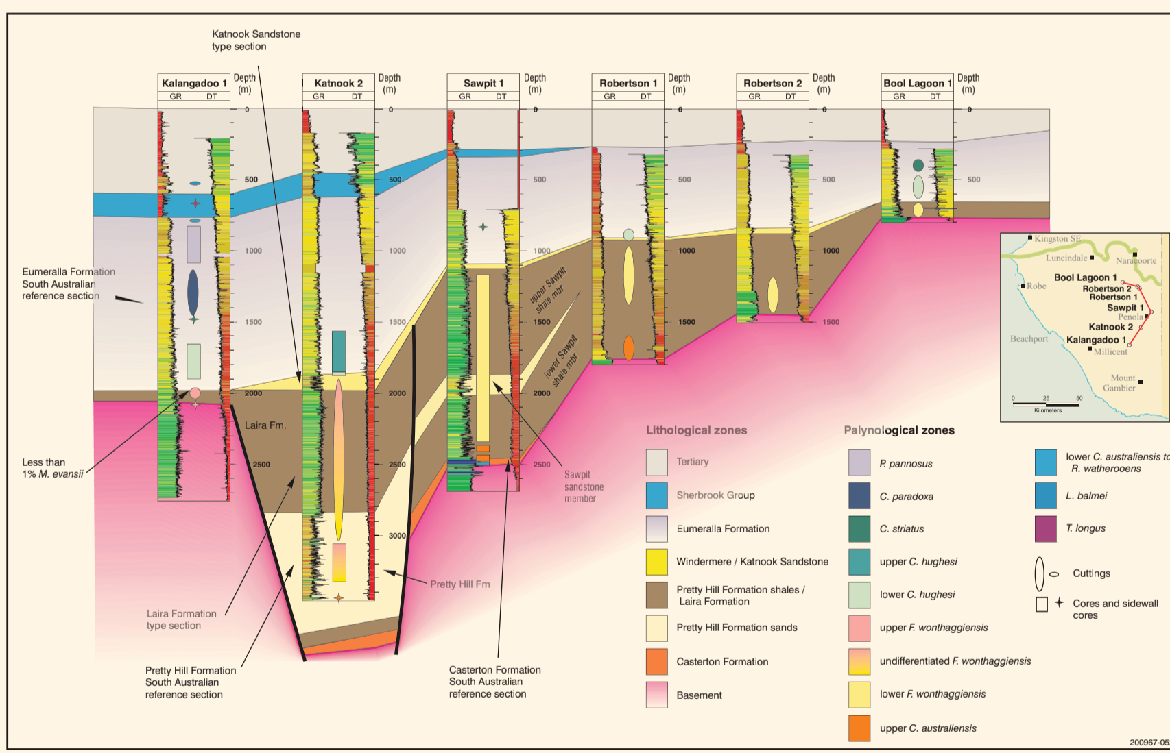
Wireline log Kalangadoo 1 to Bool Lagoon 1
