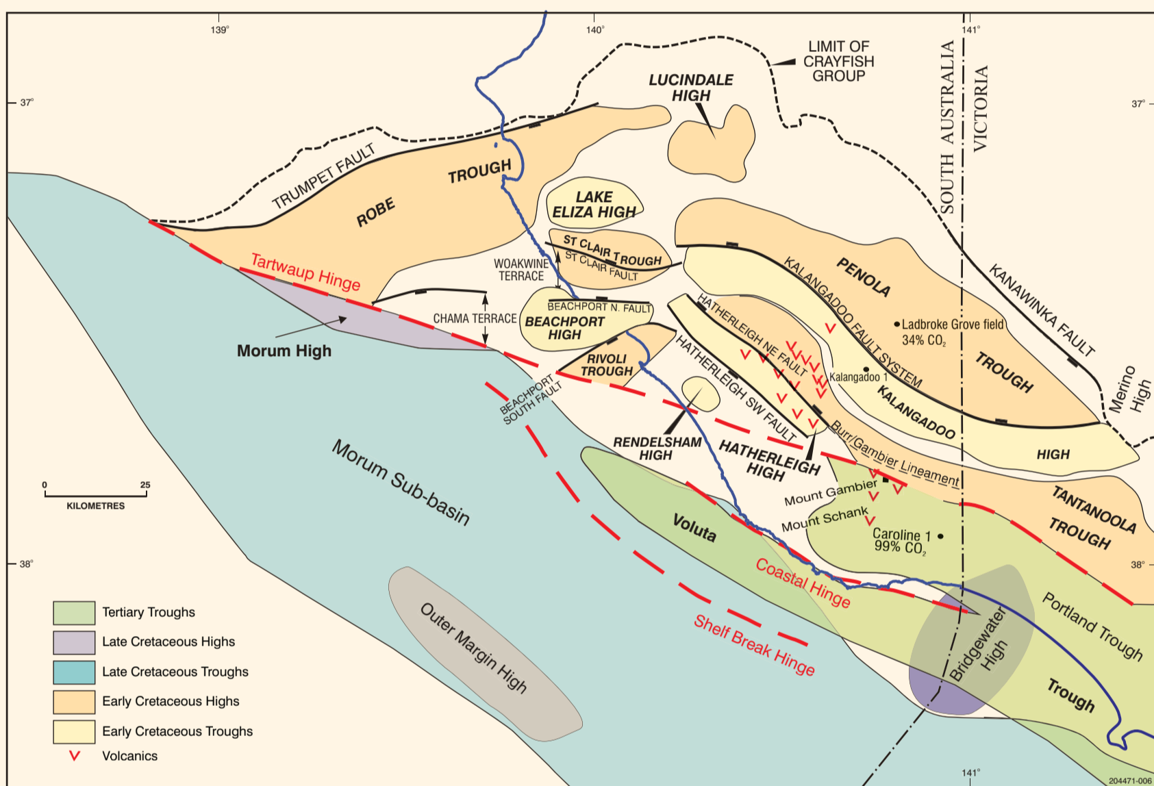
Structural elements - Otway Basin
