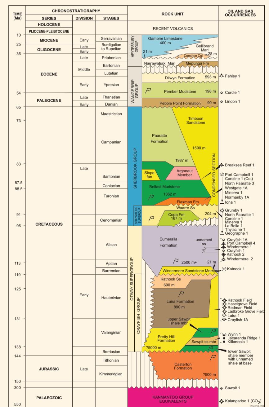
Stratigraphic column - Otway Basin
