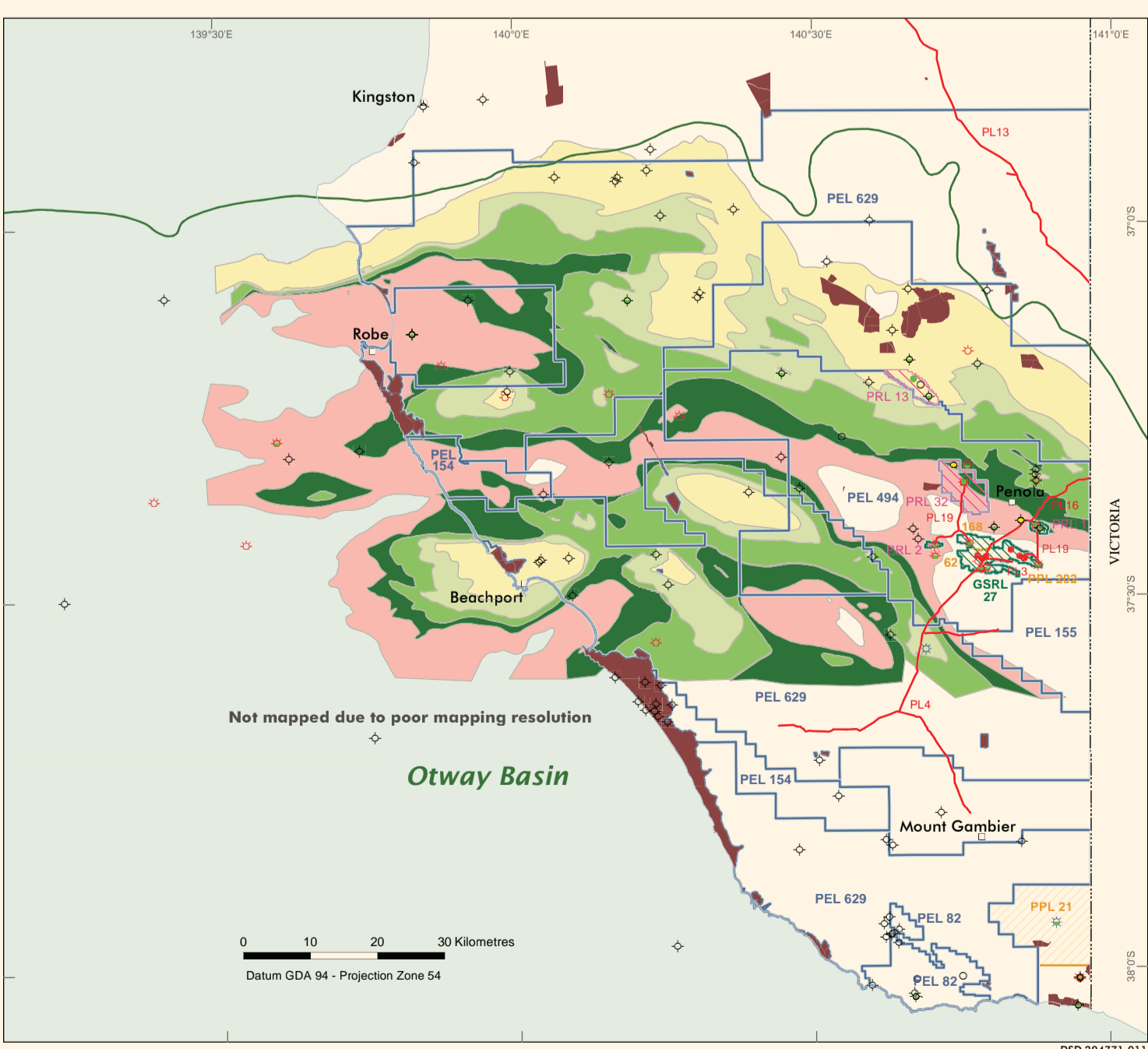
Maturity at Basement - Casterton - Base Pretty Hill Formation
